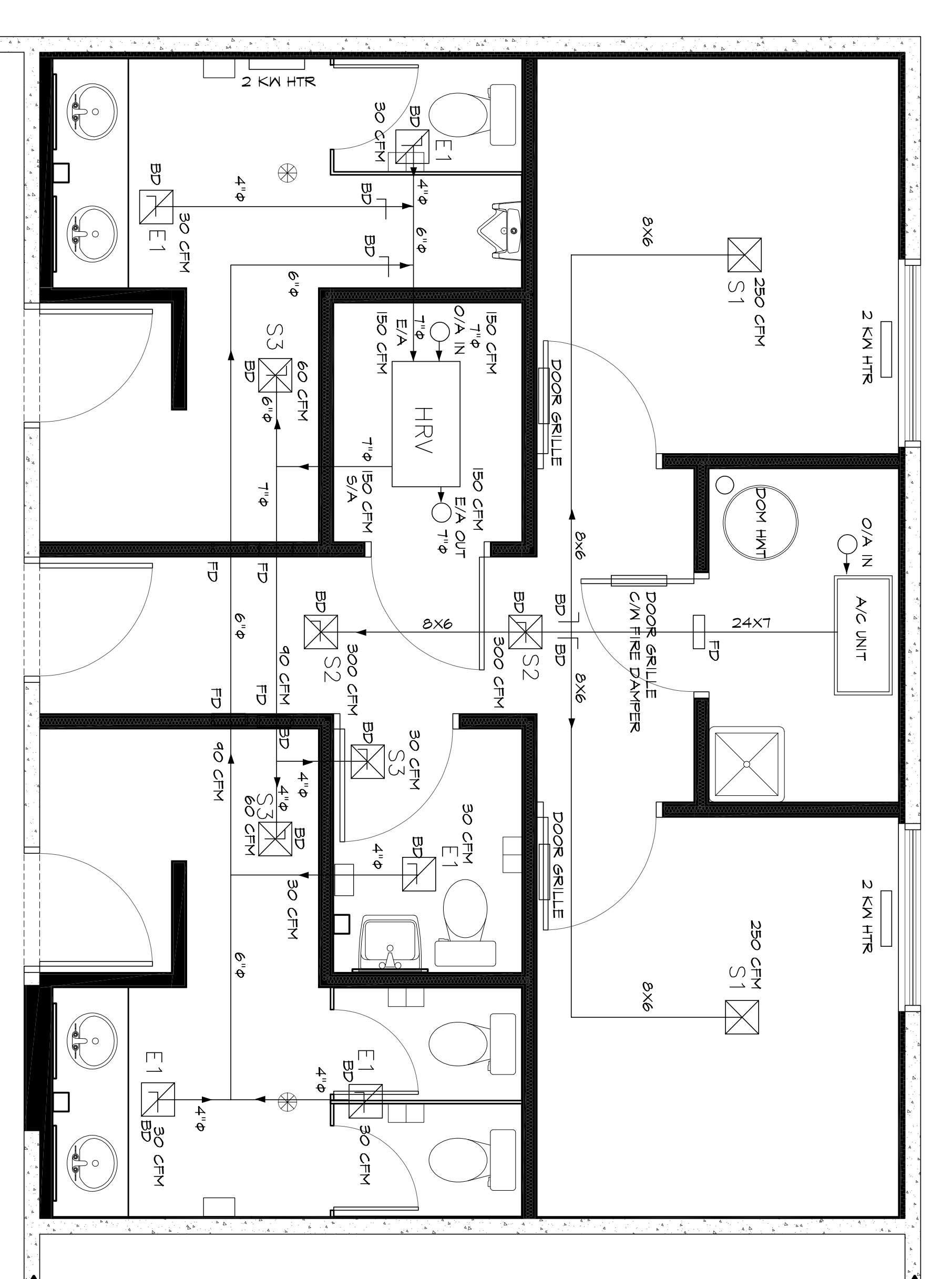
3 FLOOR PLAN - HVAC SYSTEMS SCALE: 3/8" = 1'-0"
