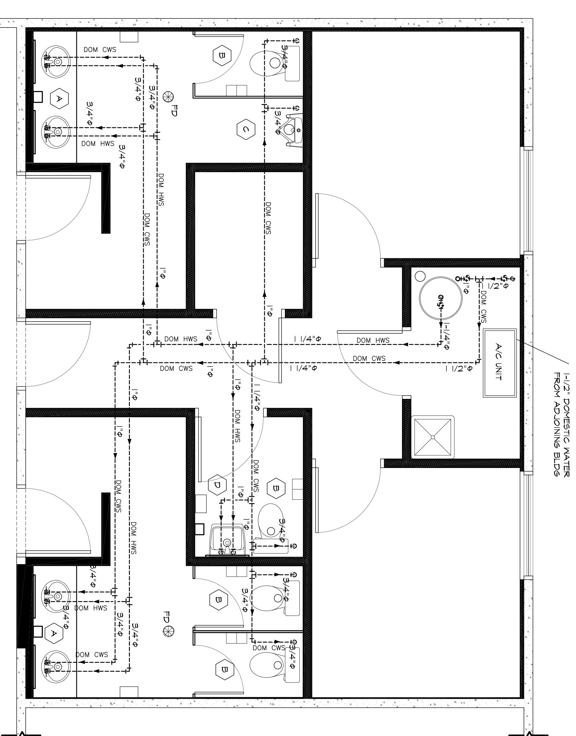
1 FLOOR PLAN - DOMESTIC WATER SCALE: 3/8" = 1'-0"
